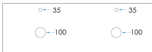
DOUBLE CUT OUT Available for sizes 1500mm-1800mm
